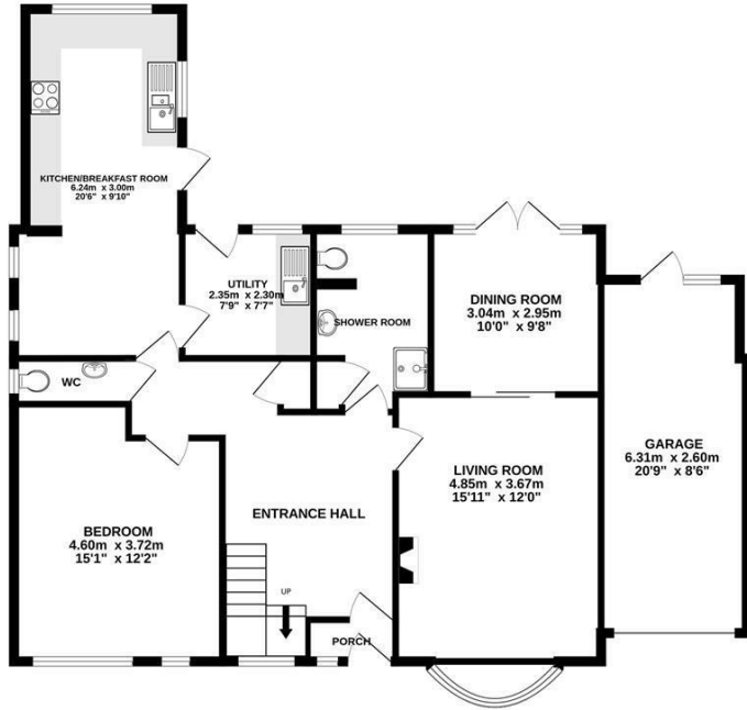
GROUND FLOOR 108.8 sq.m. (1172 sq.ft.) approx.
